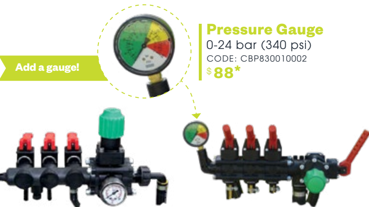
Arag Regulator & Gauge 3 Manual Section Valves CODE: ATRA10B080X3M3 $387*
